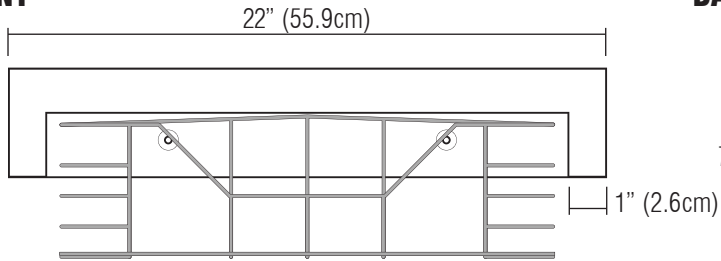
FRONT
