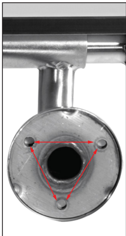
2" from center to center Flanges are 3" in diameter Holes are 0.25" in diameter
